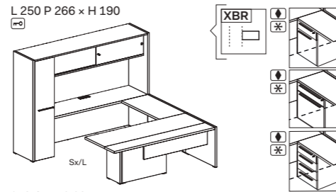
910.CM.P2.20_ Dx/R - Sx/L 910.CM.P2.22_ Dx/R - Sx/L
